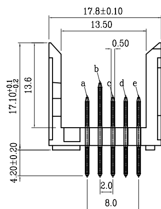
Press-fit pins
