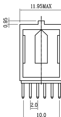
Solder pin
