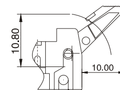
Short latch
