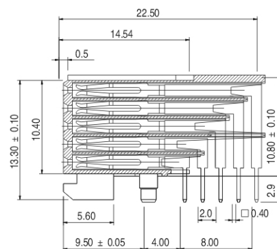
Solder pin
