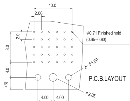
Solder pin
