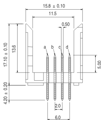
Press-fit pins
