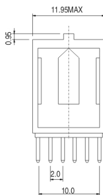
Solder pin
