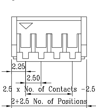
Housing
