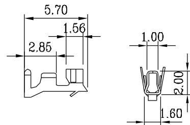
Contact
