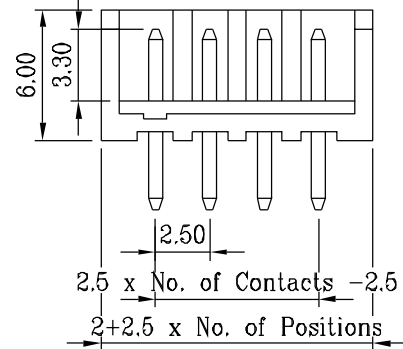
Wafer
